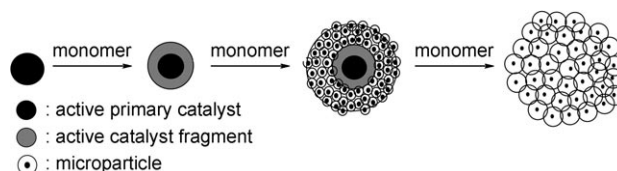
Figure 1. Fragmentation process of a pure silica catalyst (the pure “core” of a core–shell catalyst).
